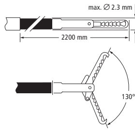
remOVE Grasper
