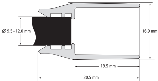
remOVE SecureCap 12
